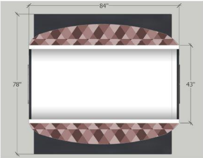
Mobile Kiosk Top Elevation
