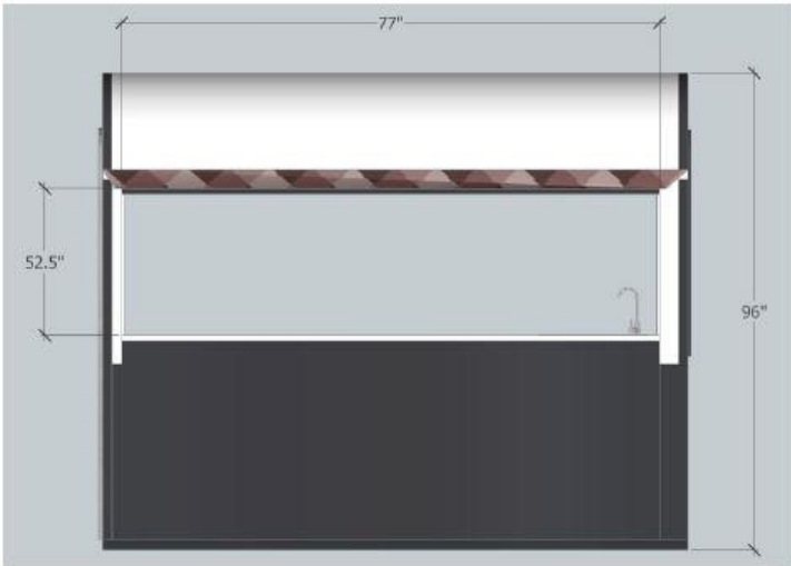
Mobile Kiosk Side Elevation
