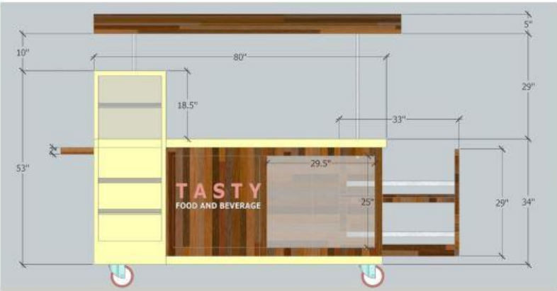
Mobile Kiosk Front Elevation
