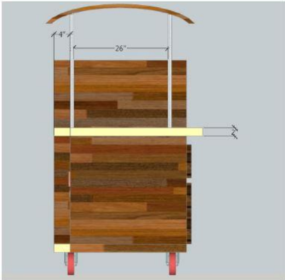
Mobile Kiosk Side Elevation
